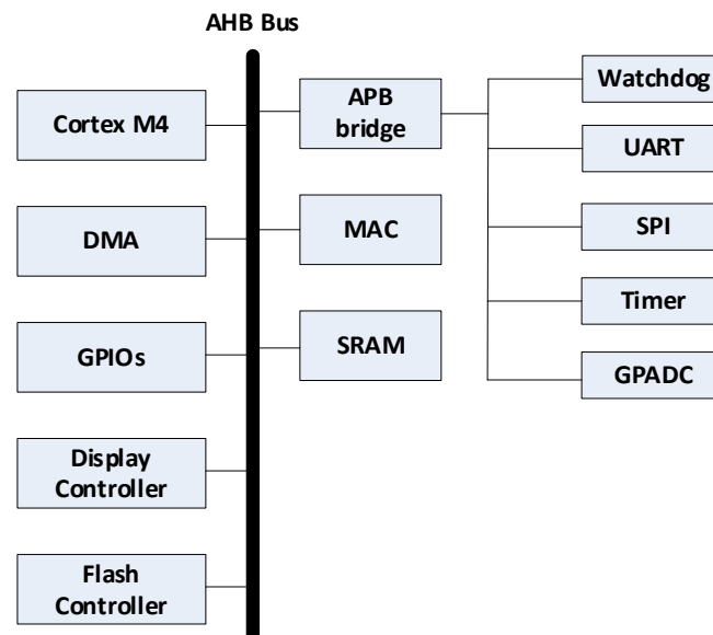
Figure 3.1 Micro-controller Subsystem
